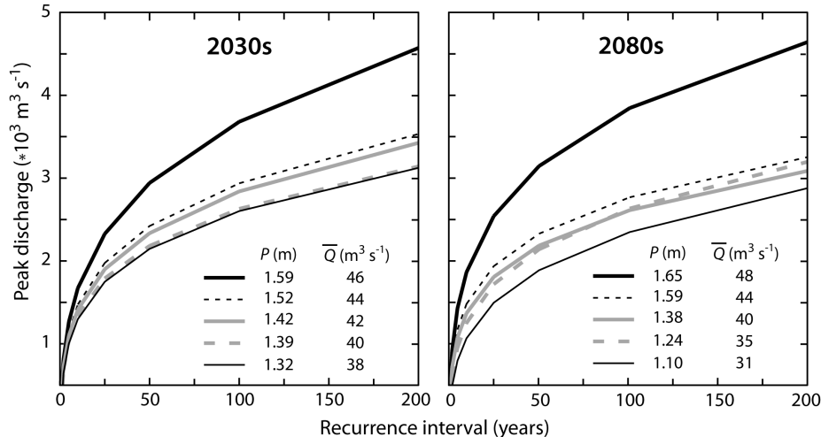
Fig. 3 Simulated log-Pearson type III peak discharge frequency curves and associated average discharge ( \bar{Q} ) for the Waipaoa River at Matawhero for the 2030s and the 2080s assuming the forecast change in precipitation ( P ).
